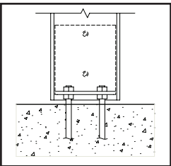
Base plate mounting detail.
