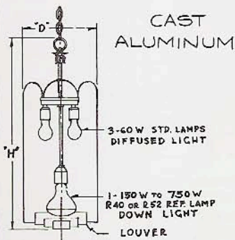
LAMP DIAGRAM LPI-308
