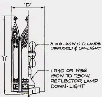
LAMP DIAGRAM - LPI-345-13
