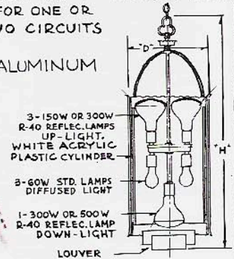
LAMP DIAGRAM LPI-304-13
