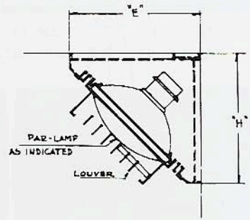
CROSS SECTIONS GC-46 AND GC-64 UNITS
