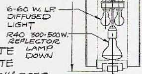
LAMPING DIAGRAM LPI-352-13
