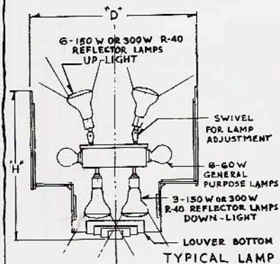
TYPICAL LAMP DIAGRAM LPI-534-28 (SHOWN)
