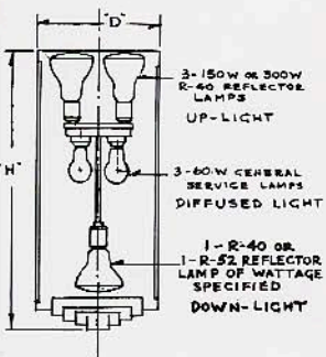
LAMP DIAGRAM LPI-577-15
